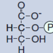
2-Phosphoglycerate
