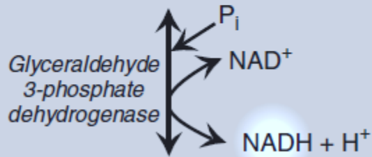
Glyceraldehyde 3-phosphate
