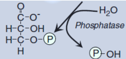
3-Phosphoglycerate
