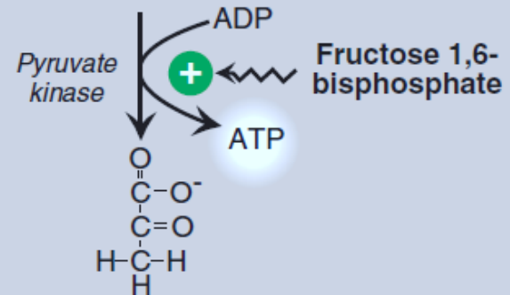
Pyruvate
