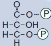
1,3-Bisphosphoglycerate
