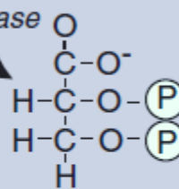
2,3-Bisphosphoglycerate
