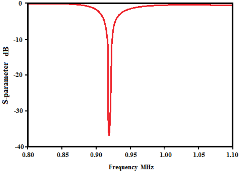
Fig.8 S-Parameter of the proposed tag antenna
