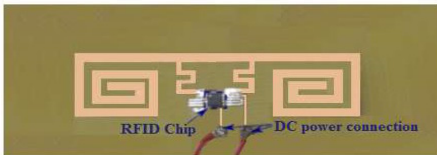
Fig. 3. Antenna of the RFID communication system.
