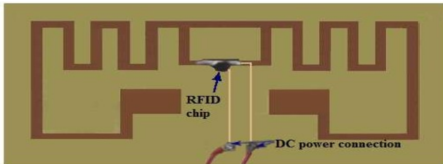
Fig. 4. Proposed antenna.
