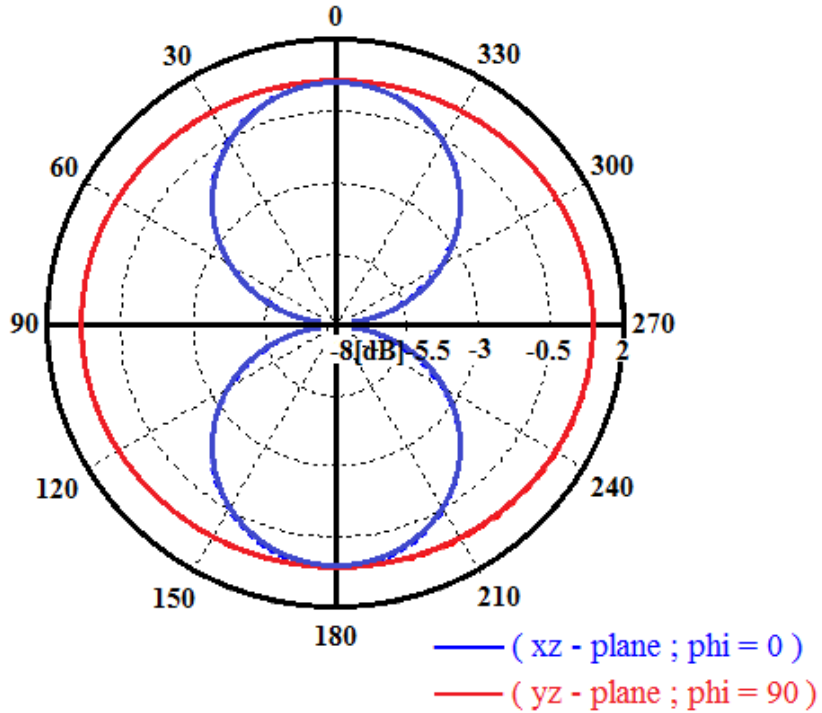
Fig.11. Polar radiation pattern of the proposed antenna
