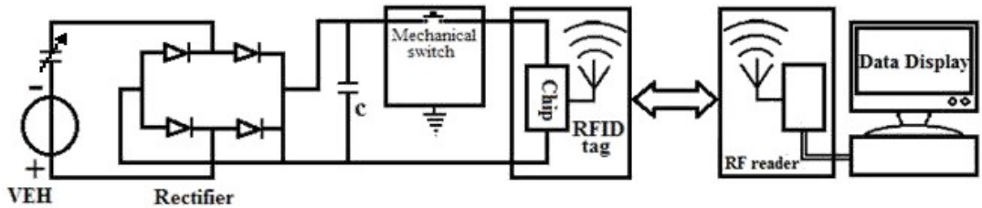
Fig. 2. Diagram of the RFID communication system.
